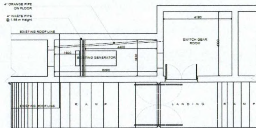
GEN-SET REHABILITATION EXISTING FLOOR PLAN SCALE 1:100 mm
