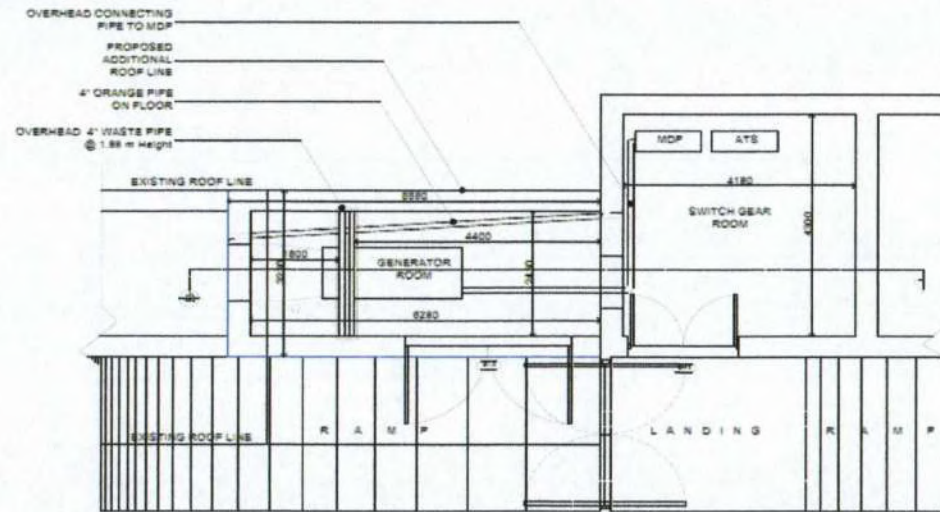
GEN-SET REHABILITATION FLOOR PLAN
